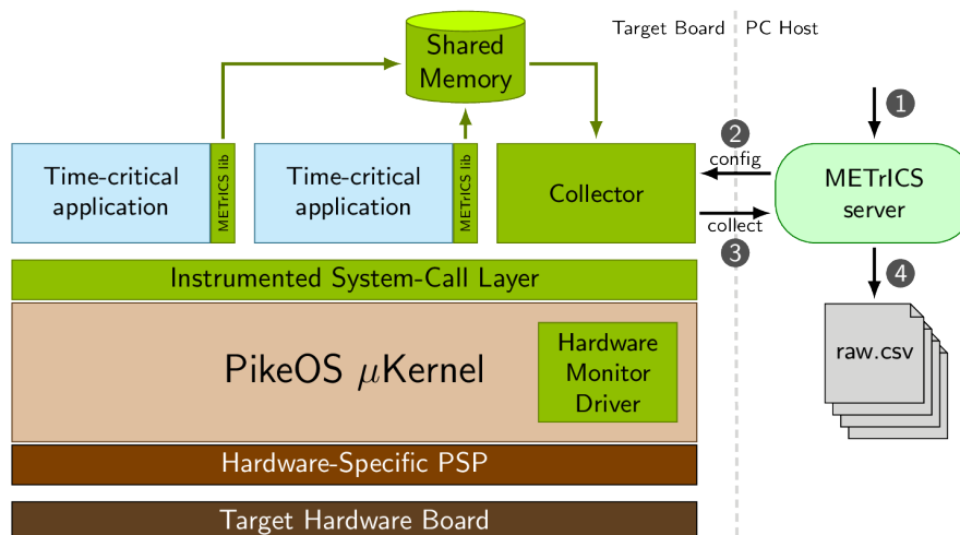
Figure 9: Architecture of the METRICS measurement tool
