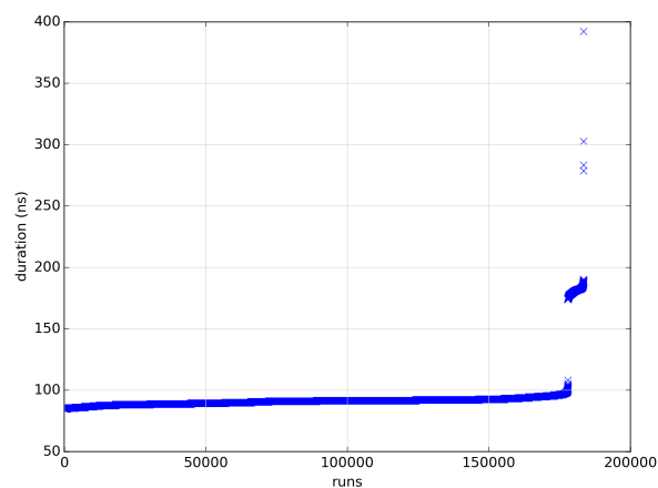
Figure 10: Completion time of a METRICS probe over 180000 runs
