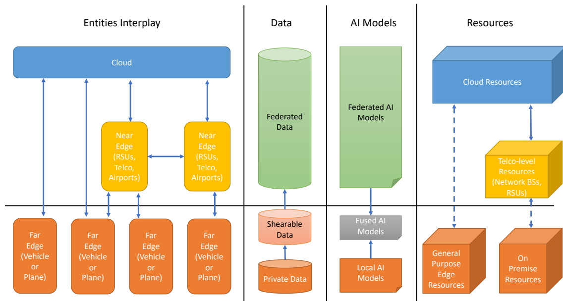
Figure 2 - Conceptual Architecture of HPC 2 I
