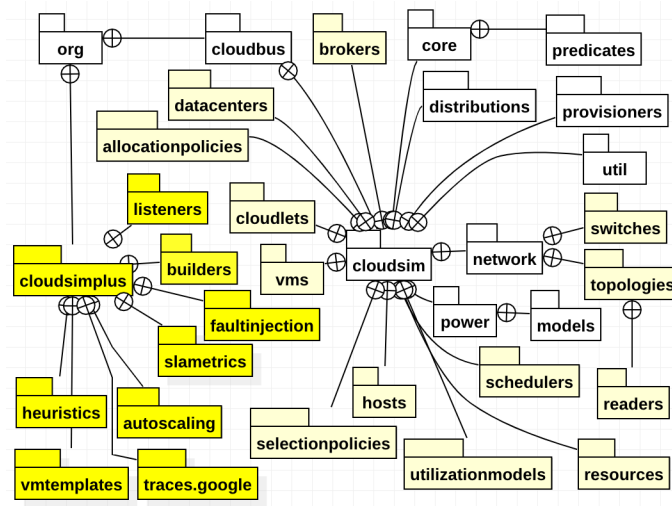
Figure 5 The modular architecture of CloudSim Plus
