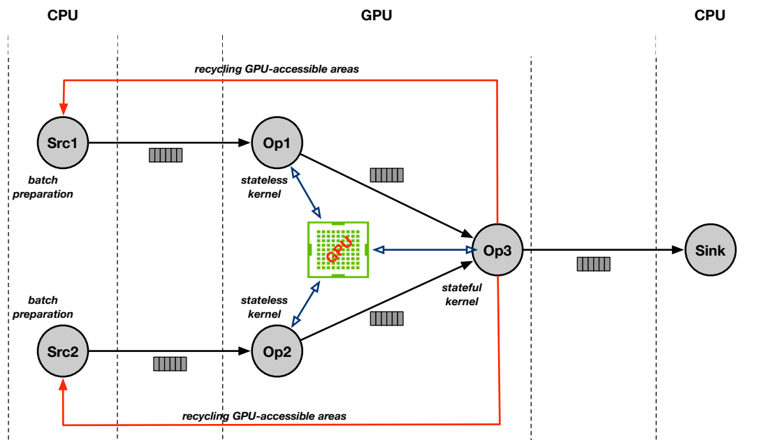
Figure 7 – Streaming on heterogeneous systems with multi-core CPUs and integrated GPUs
