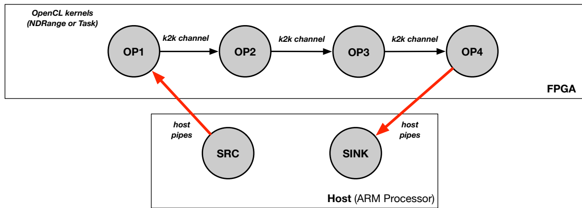
Figure 8 - Streaming on a SoC composed of an ARM processor and an Intel FPGA
