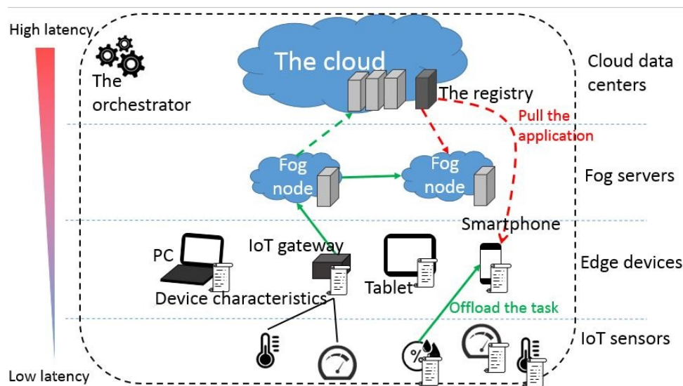
Figure 6 Architectural overview of PureEdgeSim
