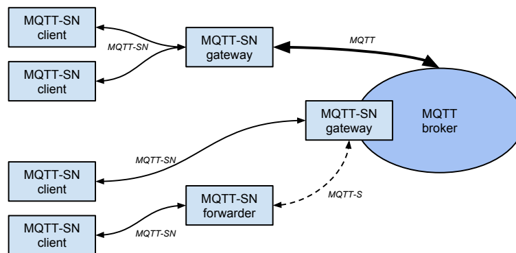
Figure 12 MQTT-SN architecture.
